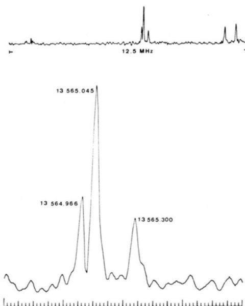
Fig. 1. Section of 1.5 MHz below a 12.5 MHz recording near the 4_{23} - 3_{22} transition of \text{CH}_3\text{CH}_2\text{NCS} . Temperature -60^\circ\text{C} , pressure 0.4 mTorr. Data acquisition: 1024 data points filled with zeros up to 4096 data points, 20 ns sample interval, time domain averaging 2^{18} cycles, frequency domain averaging 30 cycles, spectral point distance 12.5 kHz, line frequencies by three point interpolation.
